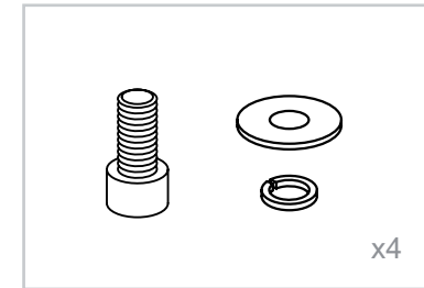
Screws (M8 x 20mm) & Gaskets
